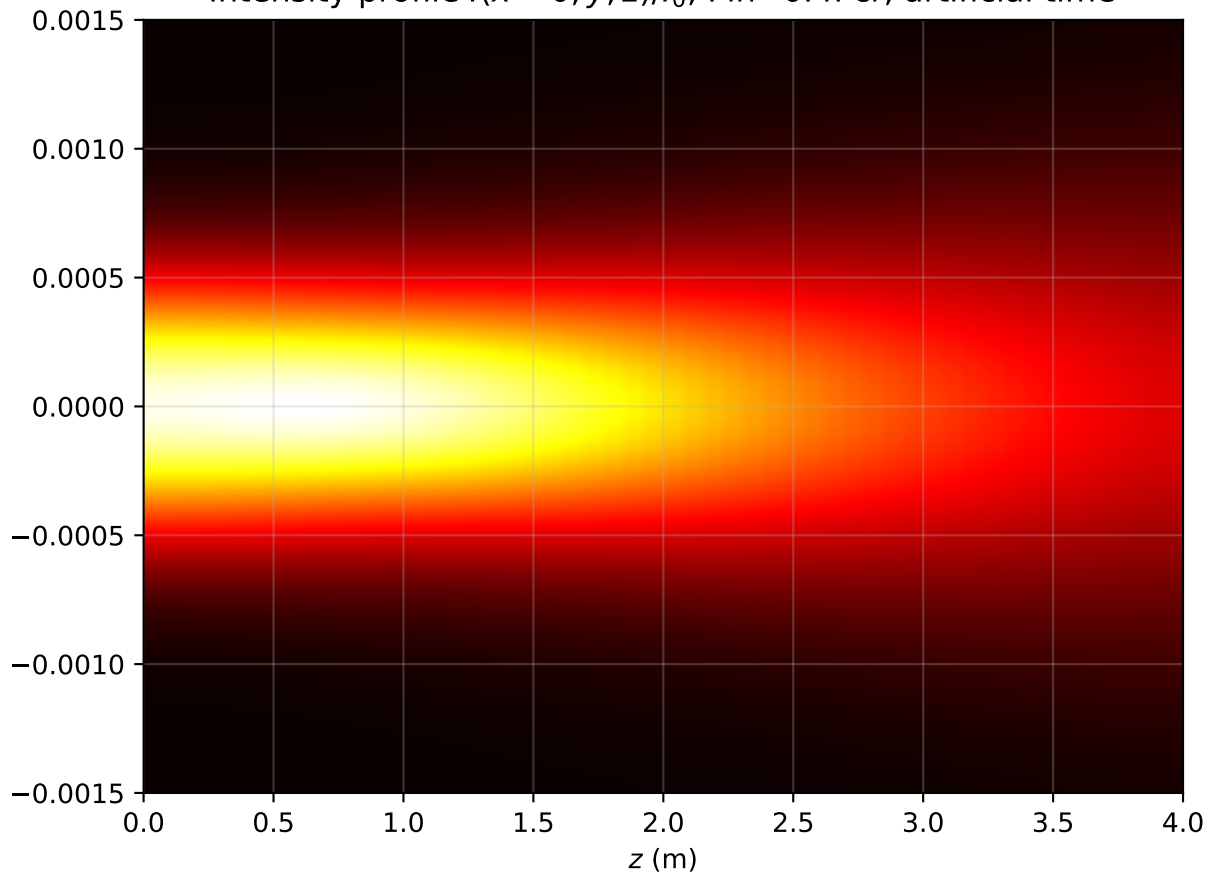
Intensity profile I(x=0, y, z)/I_0 , P_{in}=0.4P_{cr} , artificial time
